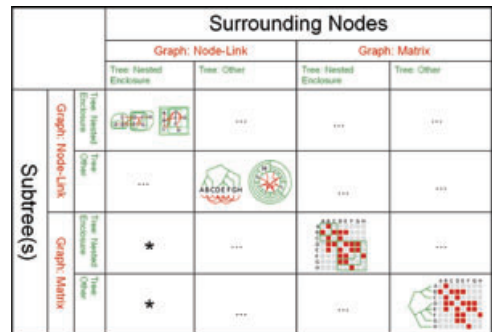
Figure 8: Hybrid visualizations of compound graphs. The TreeMatrix in Figure 9 (middle) corresponds to the two cells in the lower left corner shown here containing stars (*’).
