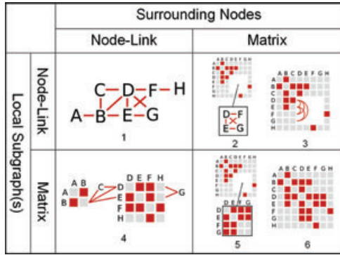
Figure 6: Hybrid visualizations of graphs. 1 shows a node-link diagram, and 6 shows a ‘pure’ adjacency matrix. 4 shows NodeTrix [HFM07], and 2, 3 and 5 show other possible hybrids.
