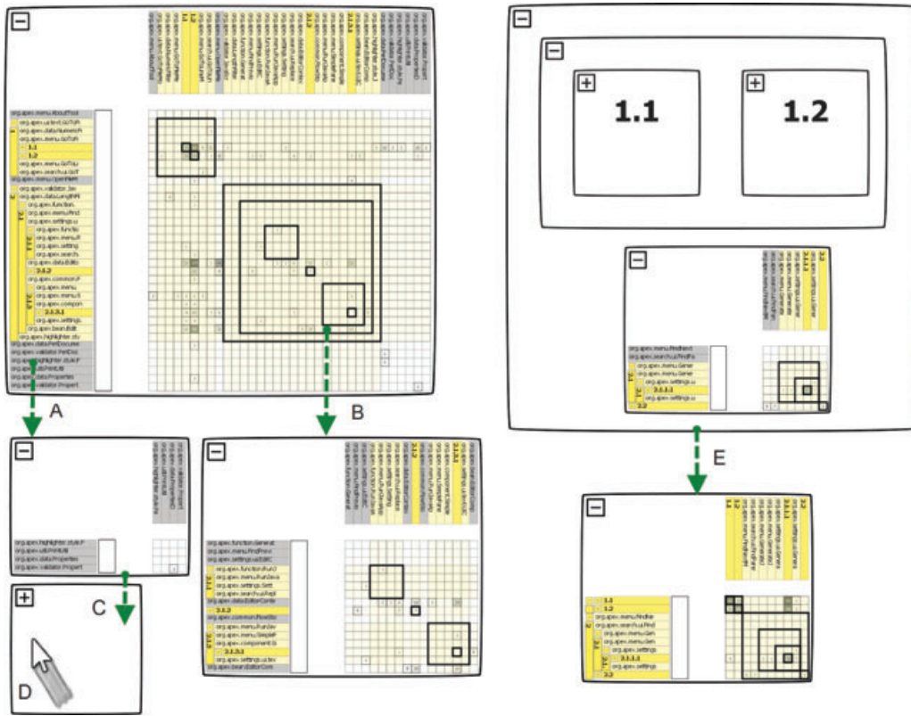
Figure 10: Moving nodes and changing their representations. (A) the user may select a subset of nodes (in this case, the last four nodes), and move them into a destination rounded rectangle by selecting 'Move Here' in the radial menu (in this case, creating a 4 \times 4 matrix). (B) the user selects one subtree within the matrix (by moving the cursor over the corresponding square) and selects 'To Matrix' in the radial menu, causing the subtree to be extracted as a new, smaller matrix. (C) Dragging an existing matrix or rounded rectangle inside another rounded rectangle causes the dragged cluster to be re-parented under the dropped location. (D) Dragging an existing matrix or rounded rectangle towards the border of its parent rounded rectangle has one of two effects: if dragged towards its parent, the parent increases in size and continues to contain the child; if dragged towards another parent, the child is allowed to leave the parent and is re-parented under that other rounded rectangle. (E) The user can also transform a cluster of nodes back into a matrix.
