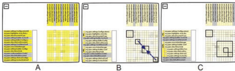
Figure 11: Creating and editing of subtrees within a matrix. (A) Initially, this matrix contains no hierarchy. The user selects four different subsets of nodes and creates a subtree for each one, shown in (B). (B) Tabs are visible along the left edge of the matrix. These form the icicle diagram showing the hierarchy, and indicate there are now four subgroups. To edit the hierarchy, the user may drag groups within their parent or into each other, resulting in (C). (C) The icicle diagram along the left edge of the matrix indicates the new hierarchical organization of groups within the matrix.
