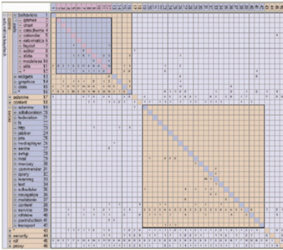
Figure 4: A screenshot of Lattix [SJSJ05].
