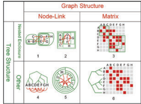
Figure 7: Non-hybrid visualizations of compound graphs showing both graph and tree structure. The lower row, labelled ‘Other’, shows tree structures using node-link or icicle diagrams. 1 is comparable to [Har88, SGJ93]. 2 is similar to [FWD*03]. 4 is similar to [PvW06], and also similar to TimeArcTrees [GBD09] if limited to only one moment in time, i.e. a node-link representation of a tree with arcs between the tree’s leaf nodes to show graph edges. 5 is similar to the radial visualization shown in [Hol06]. 3 and 6 are approaches for showing tree structure within a matrix and are similar to Lattix [SJSJ05].
