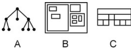
Figure 3: Three ways of drawing the same tree. (A) node-link diagram, (B) nested enclosure, (C) icicle diagram.
